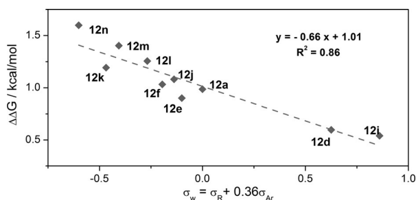
Figure 2. Correlations between the aryl substituents on the catalyst and the enantioselectivity. LFER correlating the weighted Hammett constants ( \sigma_w ) of aryl substituents with enantioselectivity. Herein, \sigma_R and \sigma_{Ar} refer to substituent constants associated with R and Ar groups, respectively. The coefficient 0.36 was obtained from a fitting procedure (see the Supporting Information).
